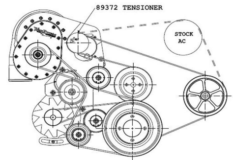
BELT ROUTING
