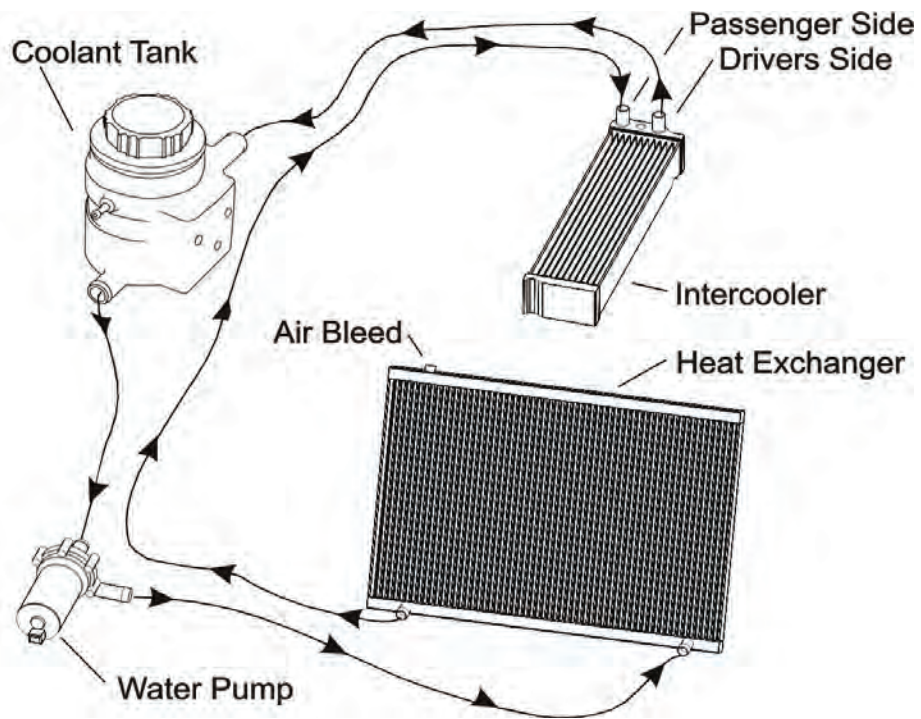
Intercooler System Diagram
