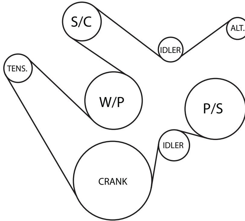
Belt Routing Diagram
