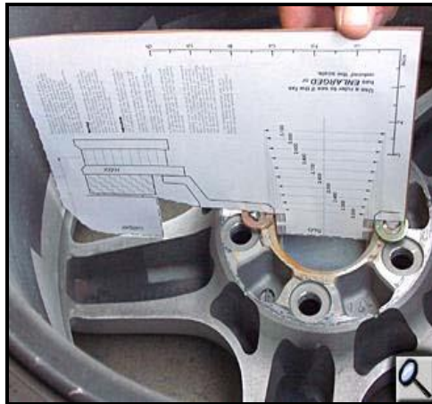
Figure 5: Washers used as temporary spacers for template clearance
