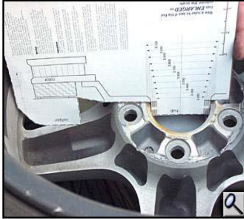
Figure 4: Template fitment
