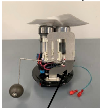
Installed "Old-Style" fuel level sender bracket on outlet cap with socket head cap screws and lock washers.
