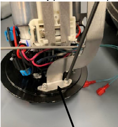
Install fuel level sender bracket on outlet cap with socket head cap screws and lock washers.
