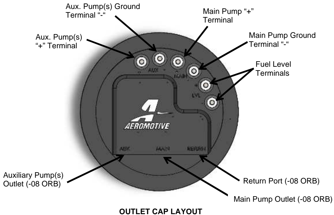
OUTLET CAP LAYOUT
