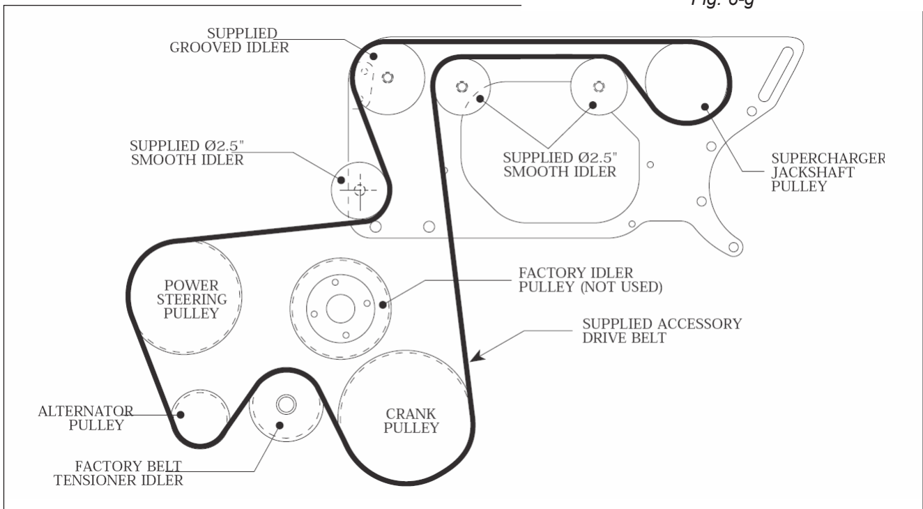
Fig. 6-e / Accessory Drive Belt Routing (300hp Engines)
