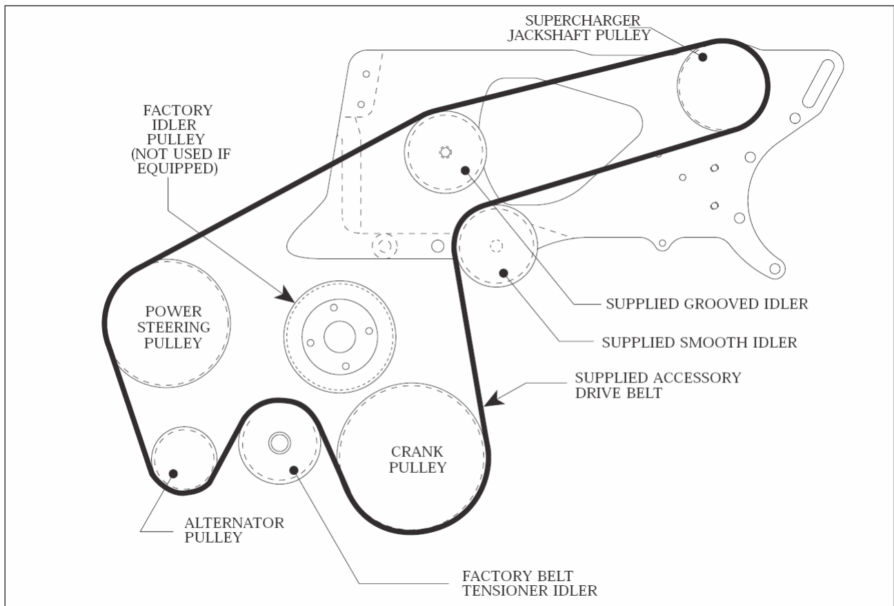
Fig. 5-e / Accessory Drive Belt Routing
