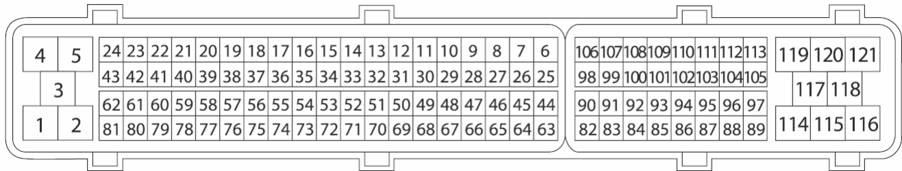
Fig. 10-c / As viewed from the back of the connector (Where the wires are inserted)
