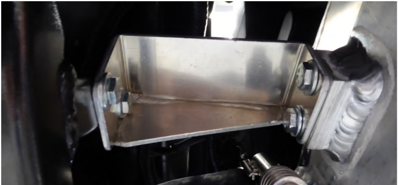
RIGHT SIDE INTERCOOLER MOUNTING BRACKET INSTALLED
