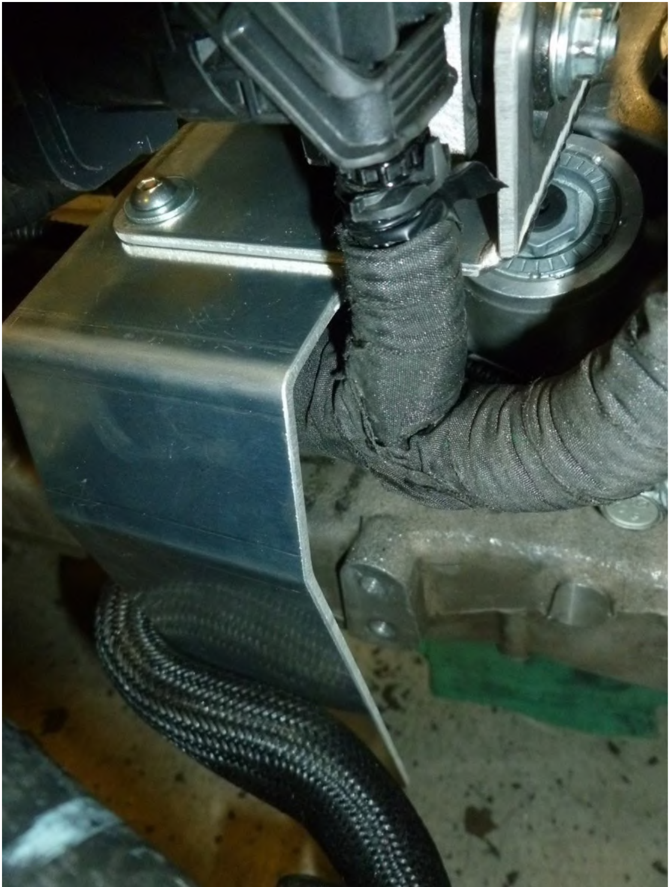
(WIRE HARNESS ROUTED BEHIND NEW ABS MODULE MOUNTING BRACKET)
