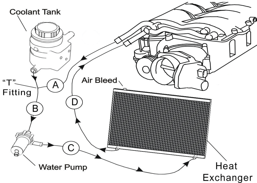
Intercooler Routing Diagram C6 Corvette Heartbeat
