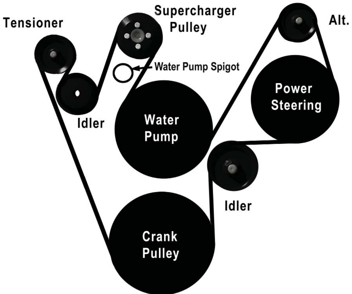
2006-2008 C6 LS7 Corvette Drive Belt Routing Diagram (Gates Belt #K061005)
