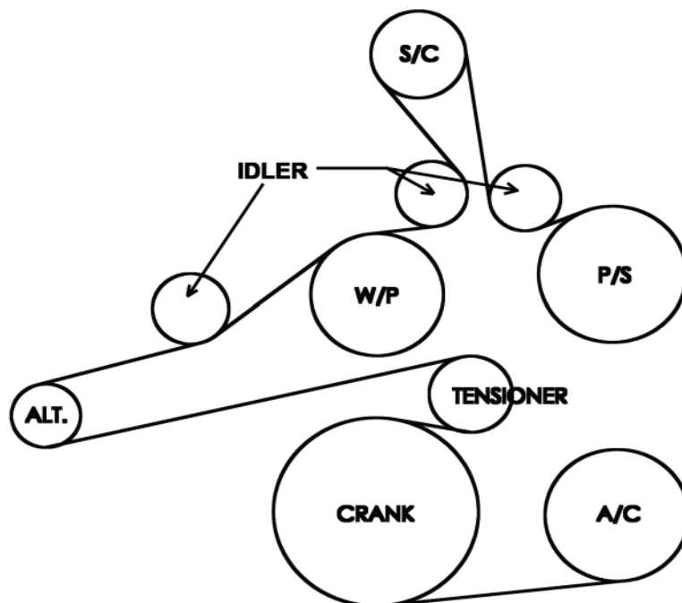
HEMI Belt Routing Diagram
