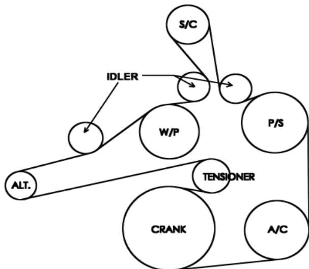
HEMI Belt Routing Diagram
